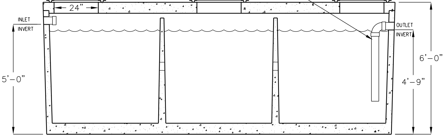
SIDE VIEW (CUTAWAY)
