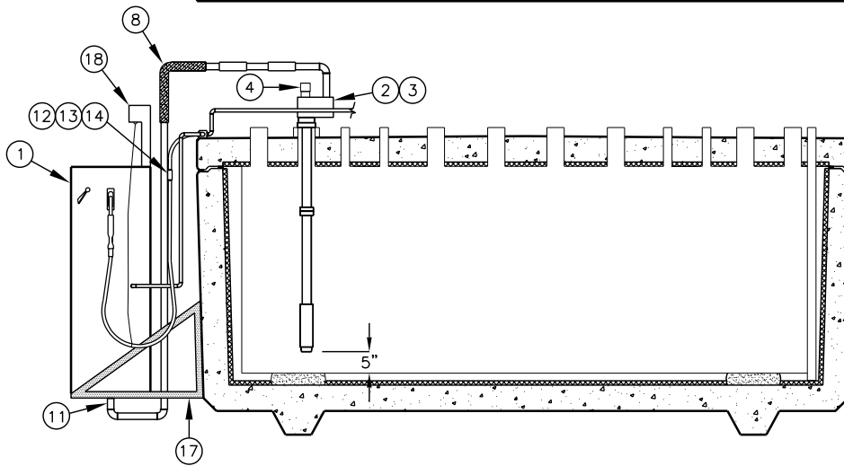
ELEVATION (CUTAWAY)
