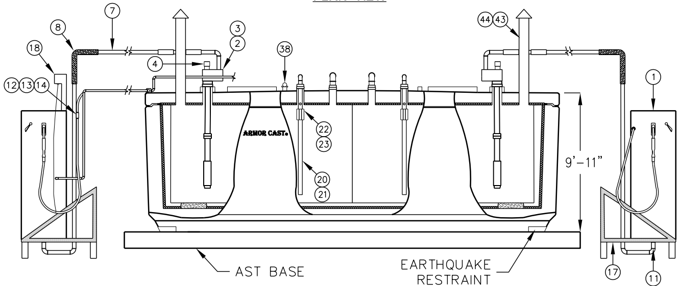
ELEVATION (CUTAWAY)
