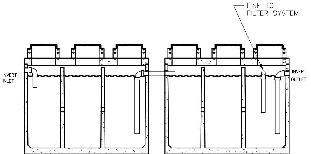
RECLAIM SYSTEM
