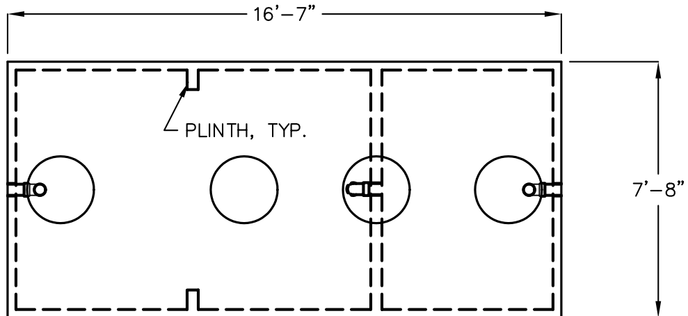
TOP VIEW (COVERS REMOVED)
