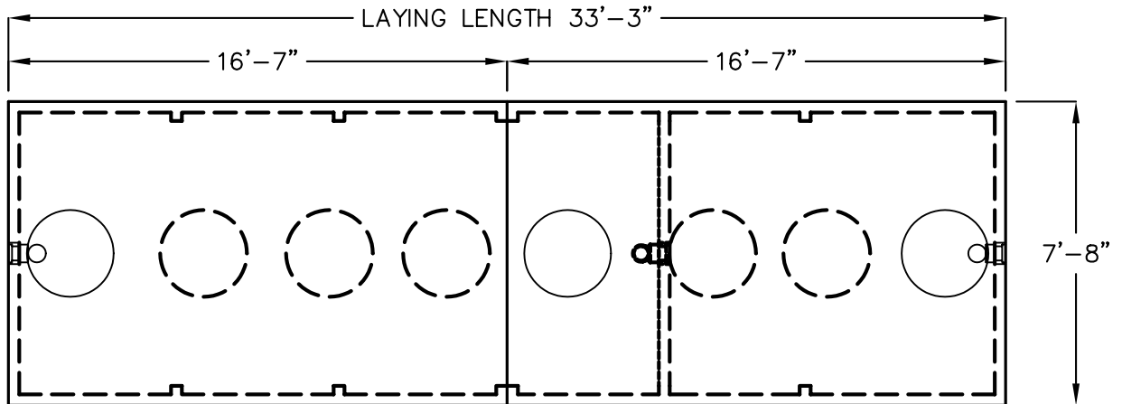
TOP VIEW (COVERS REMOVED)
