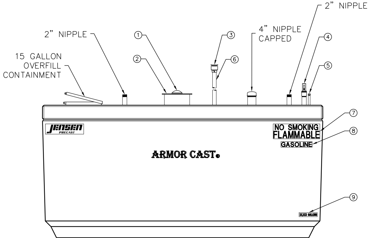
6000-12000 GALLON TANKS
