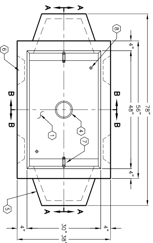
PLAN VIEW
