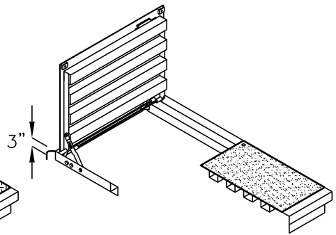
ADJUSTABLE TORSION SPRING ASSISTED COVERS (NON-SLIP SURFACE)
