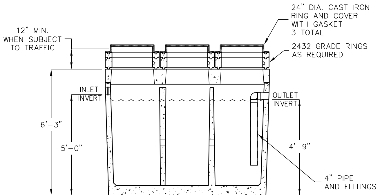
ELEVATION SECTION
