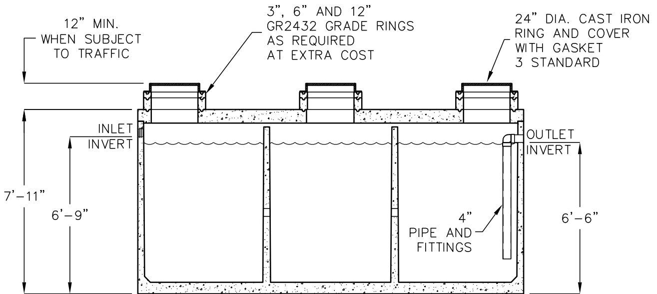
ELEVATION SECTION
